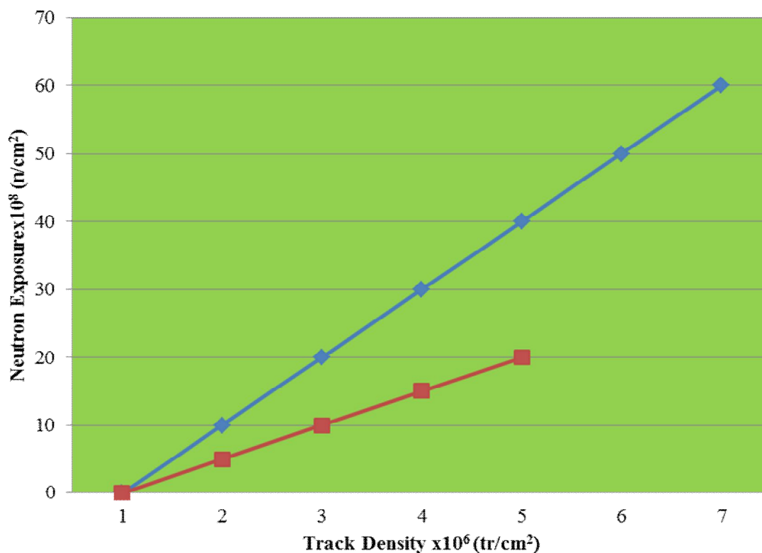
Fig. 2: Variation of track density with the neutron exposure for five minute etching time
