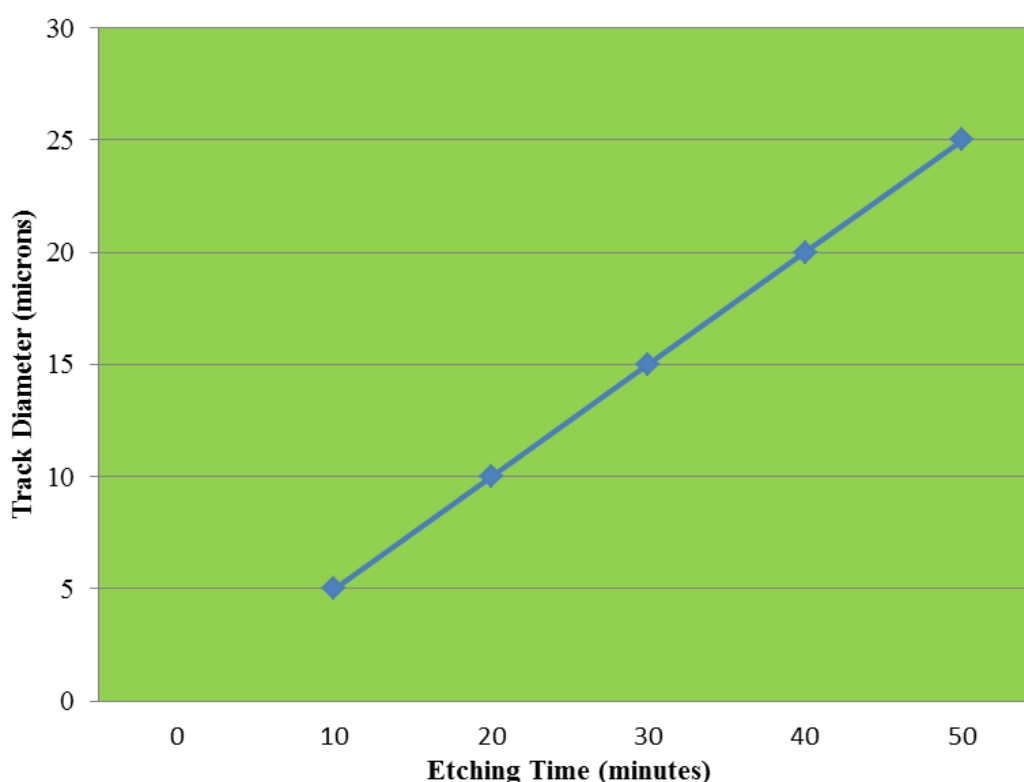
Fig.: 1 Growth of track diameter as a function of the etching time
